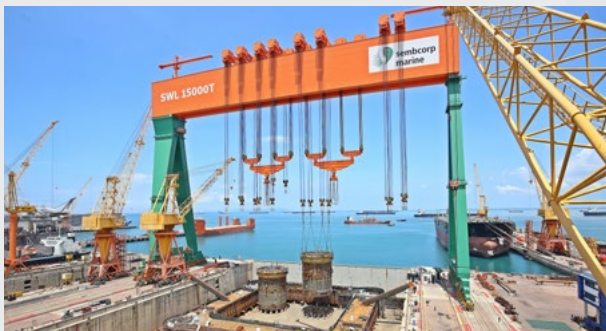
Sembcorp Marine's goliath gantry crane at Tuas Boulevard Yard lifting Shell Vito FPU columns
